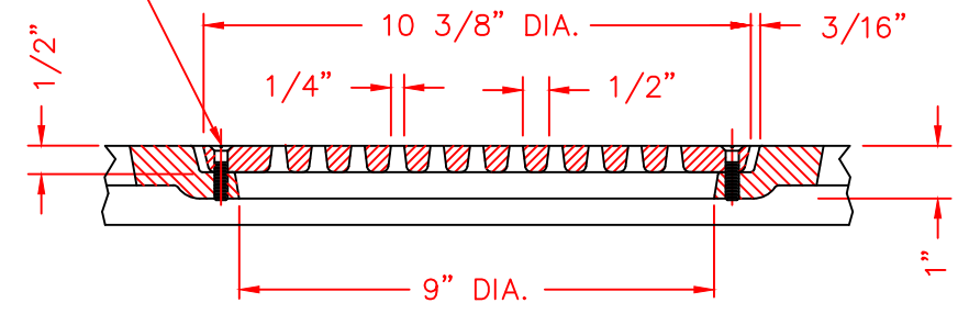
LIGHT OPENING DETAIL QUARTER SCALE
