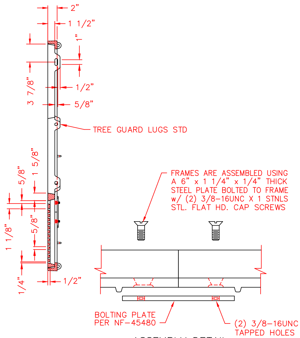
ASSEMBLY DETAIL HALF SCALE
