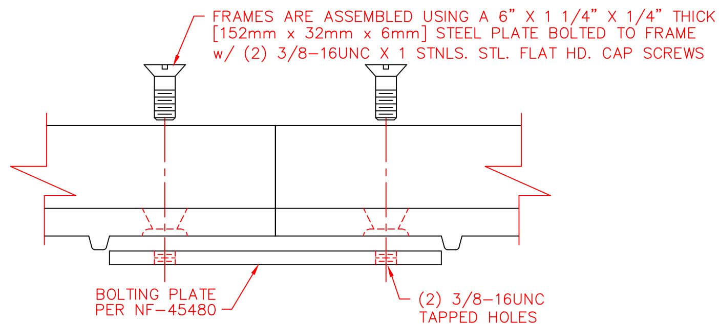
ASSEMBLY DETAIL SCALE 1:2
