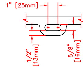
BOLT SLOT DETAIL QUARTER SCALE
