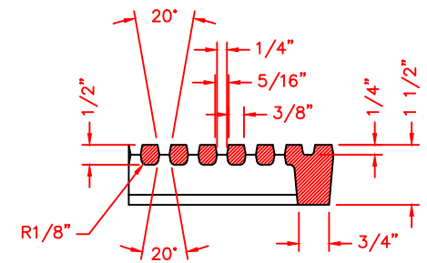
CROSS-SECTION DETAIL SCALE = 1:4
