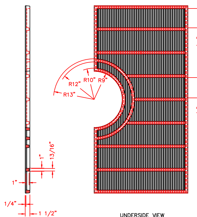
UNDERSIDE VIEW
