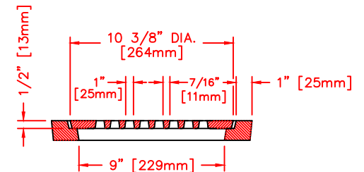
ASSEMBLY DETAIL SCALE 1:2
