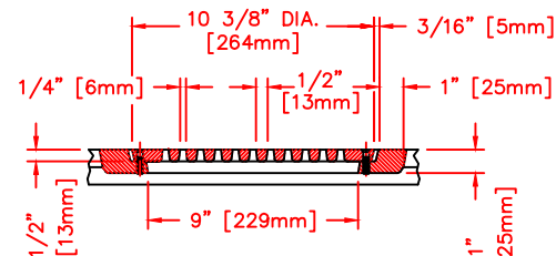
LIGHT OPENING DETAIL LIGHT GRATE COMPONENT NO. 8718-0004
