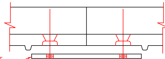
ASSEMBLY DETAIL SCALE 1:2
