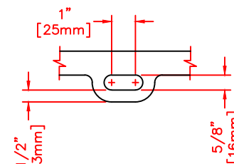
BOLT SLOT DETAIL QUARTER SCALE
