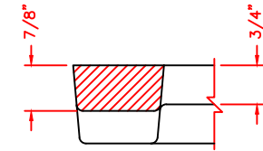
SECTION A-A HALF SCALE
