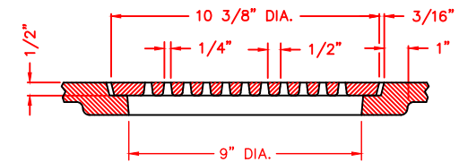
SECTION THRU LIGHT OPENING SPECIAL PEDESTRIAN SAFE LIGHT GRATE
