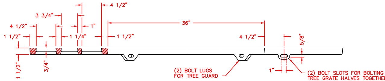
SECTION THRU LIGHT OPENING SPECIAL PEDESTRIAN SAFE LIGHT GRATE
