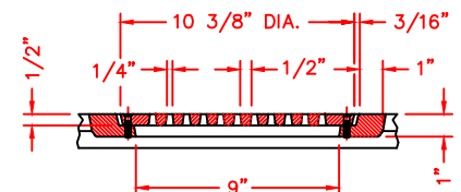
LIGHT OPENING DETAIL LIGHT GRATE COMPONENT NO. 8718-0004
