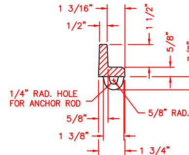
TYPICAL FRAME SECTION SCALE 1:4
