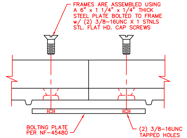
FRAME ASSEMBLY DETAIL SCALE 1:2
