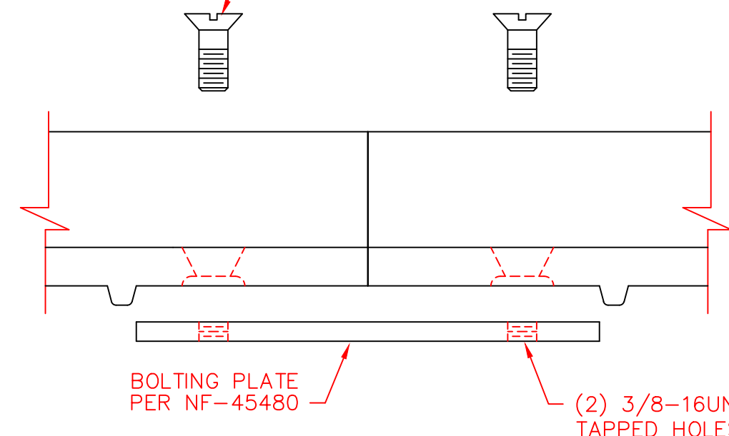
ASSEMBLY DETAIL HALF SCALE
