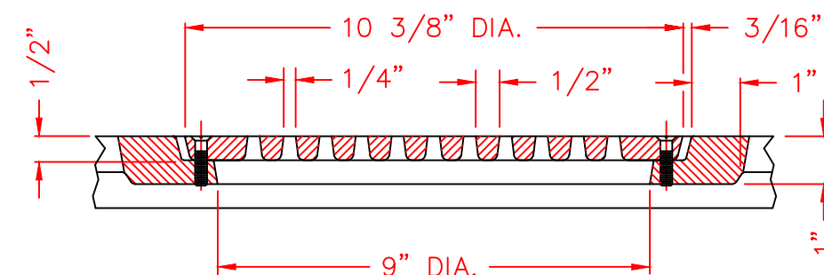
LIGHT OPENING DETAIL QUARTER SCALE
