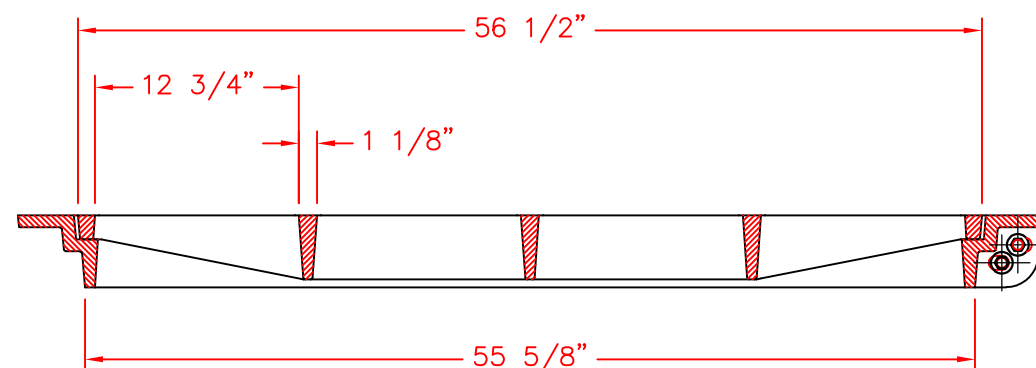
SECTION B-B
