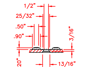
DOME & VENT DETAIL SCALE 1:2
