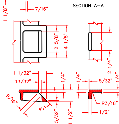
QUICK CONNECT LOCK SLOT AND LUG DETAIL SCALE 1:2 LOCK SLOT AND LUG 'A'
