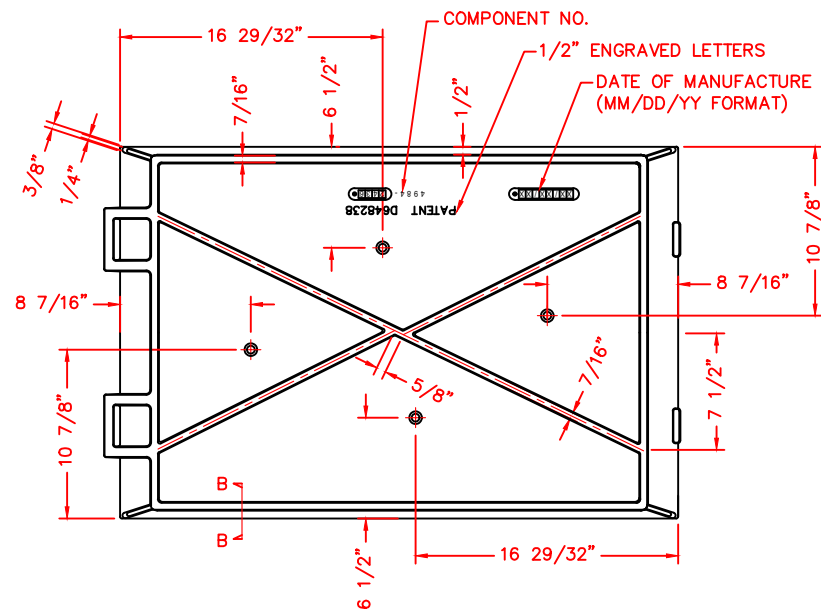
UNDERSIDE VIEW
