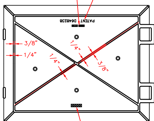
BOTTOM OF PLATE
