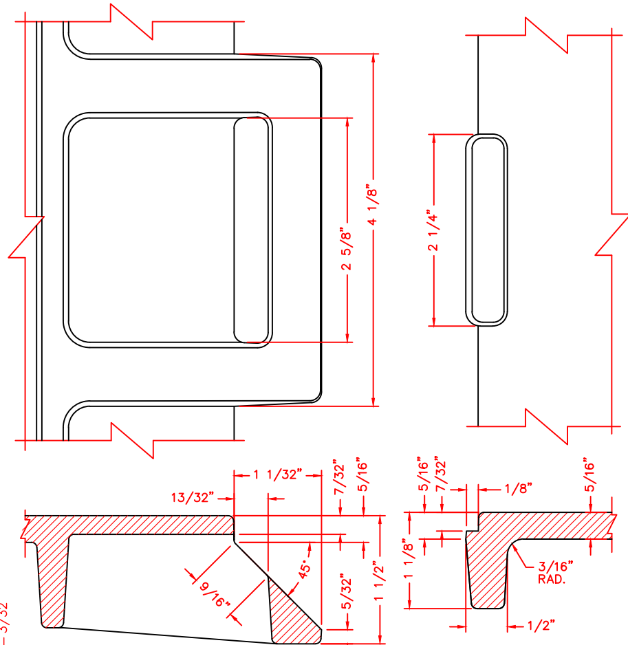
QUICK CONNECT LOCK SLOT AND LUG DETAIL FULL SCALE LOCK SLOT AND LUG
