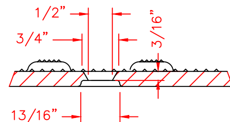
VENT DETAIL
