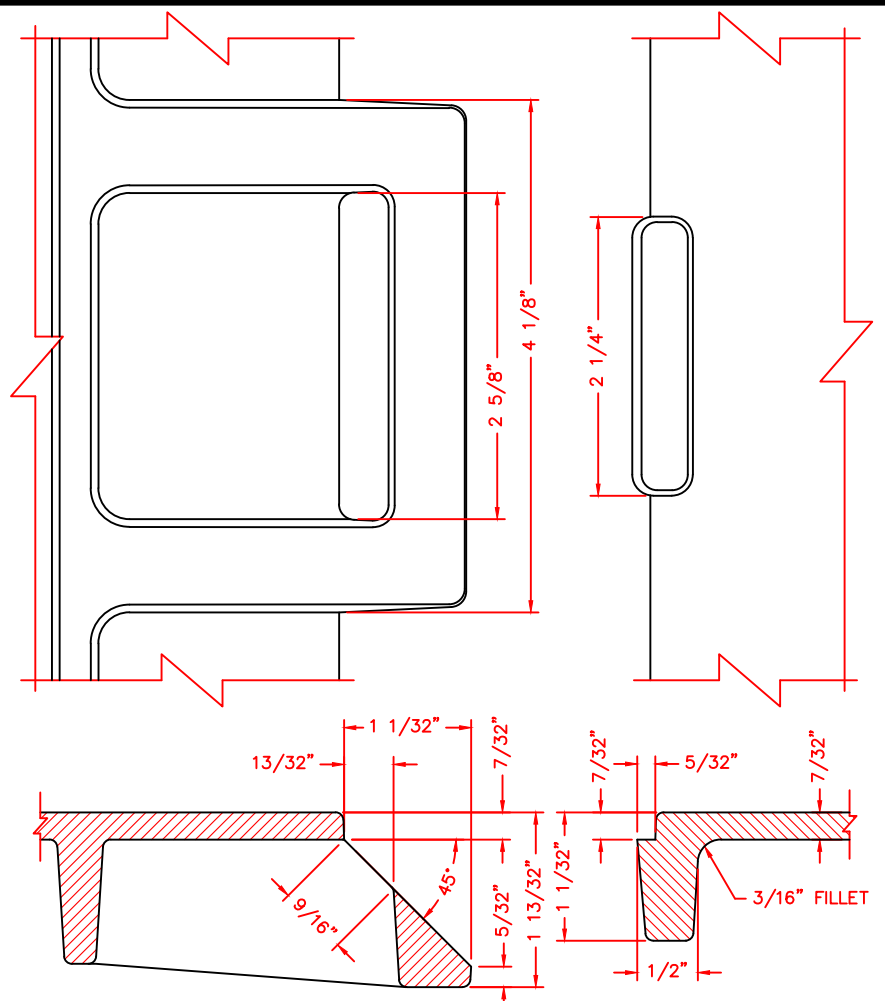
QUICK CONNECT LOCK SLOT AND LUG DETAIL FULL SCALE LOCK SLOT AND LUG 'A'
