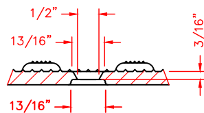
VENT DETAIL SCALE 1:2
