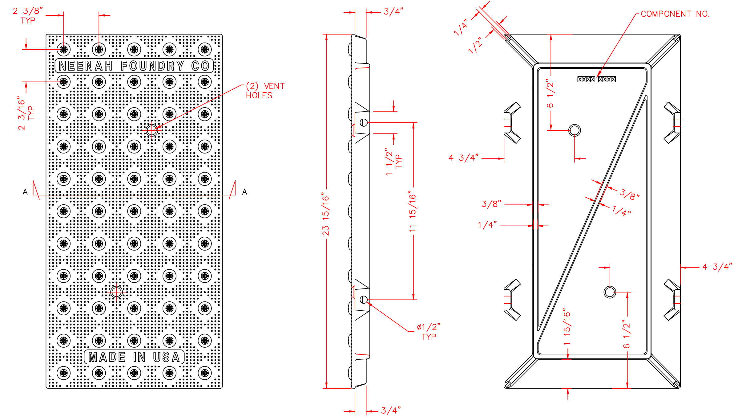
UNDERSIDE VIEW
