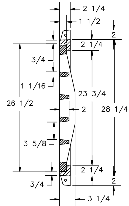
B-B SECTION
