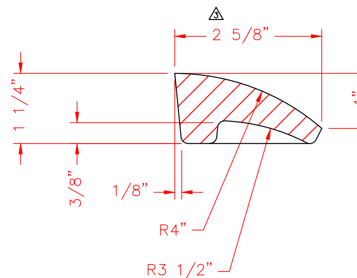
FIRST VANE DETAIL (SCALE: 1:2)
