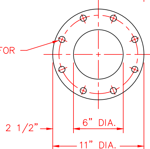
BOTTOM VIEW OF FLANGE ONLY
