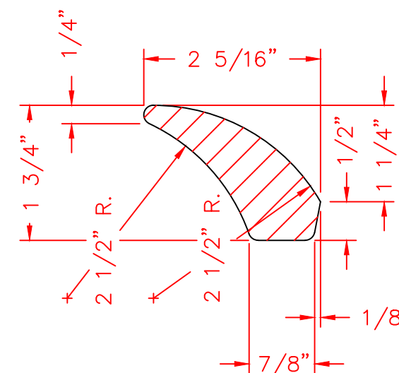
SECOND VANE DETAIL (SCALE: 1"=1/2")
