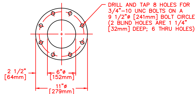
BOTTOM VIEW OF FLANGE ONLY
