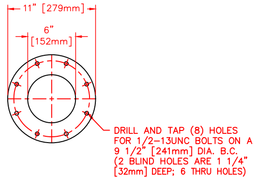
BOTTOM VIEW OF FLANGE ONLY
