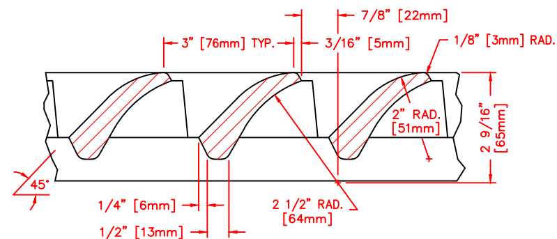
SECTION THRU VANES AND SHOWING CENTER RIB HALF SCALE
