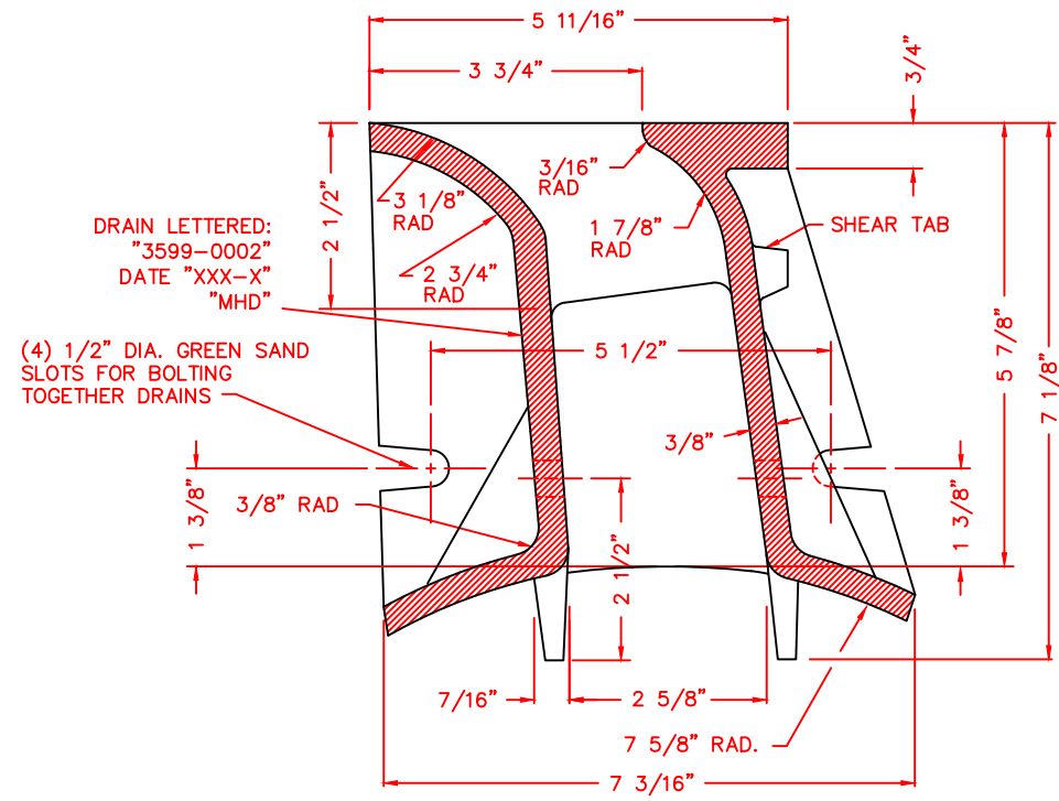
SECTION THRU VANE DRAIN HALF SCALE
