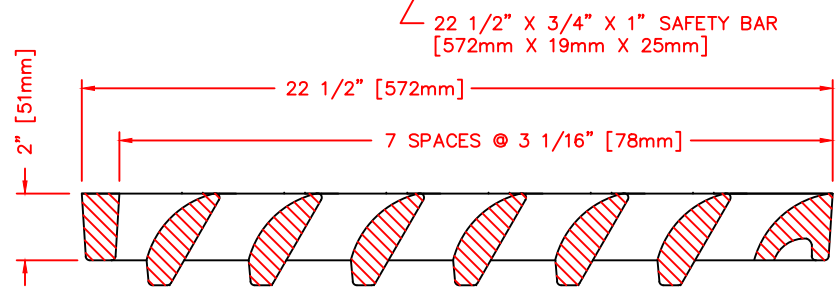
SECTION THRU GRATE ONLY
