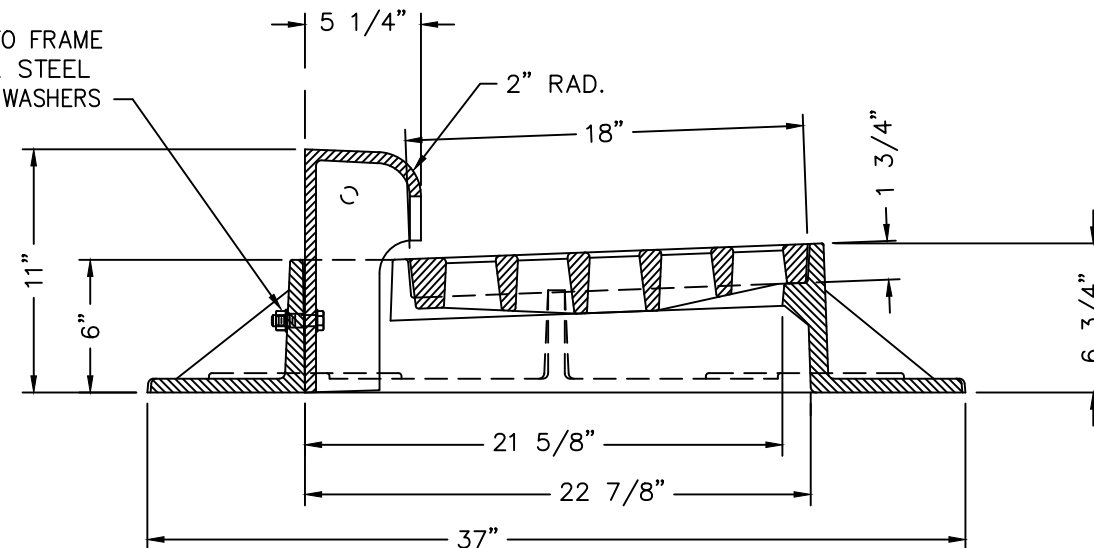
SECTION B-B
