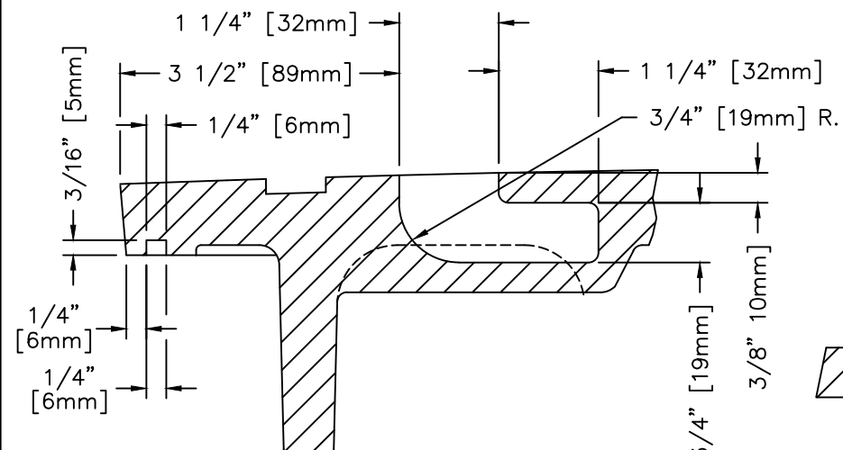
SELF-SEAL GROOVE AND CONCEALED PICKHOLE HALF SCALE
