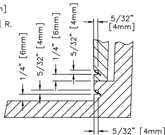
GASKET GROOVE DETAIL HALF SCALE
