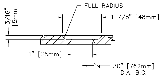
ANCHOR HOLE DETAIL SCALE 1:2
