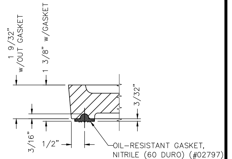
"T SEAL" GASKET DETAIL SCALE 1:2
