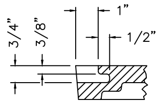
PICKHOLE DETAIL QUARTER SCALE
