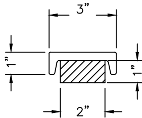
SECTION A-A QUARTER SCALE
