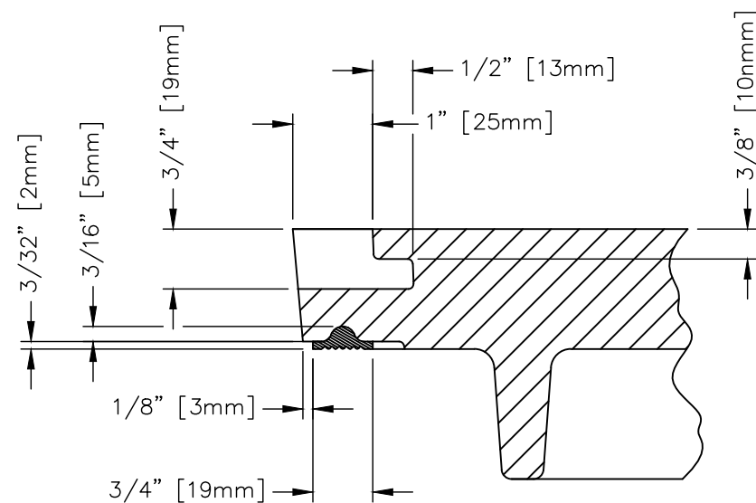
CONCEALED PICKHOLE GASKET DETAIL SCALE 1:2
