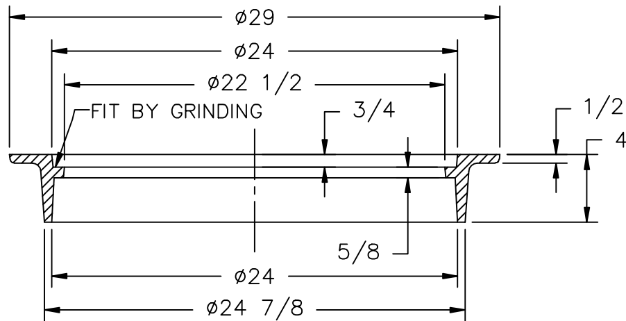
SECTION B-B (1259_RING)
