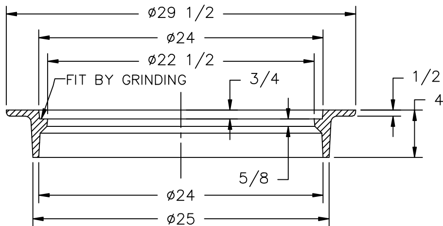
SECTION B-B (1258_RING)
