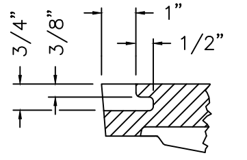
PICKHOLE DETAIL QUARTER SCALE
